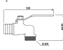
Küresel Bas Drainage Ball Tap
